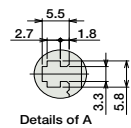
■ Dimensions and Weight by Stroke * Adding a brake will increase the actuator's weight by 0.3kg.
