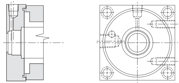
HYDRAULIC DRAIN PORT DETAIL
