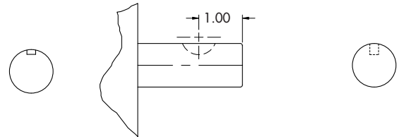
#808 Woodruff Key
